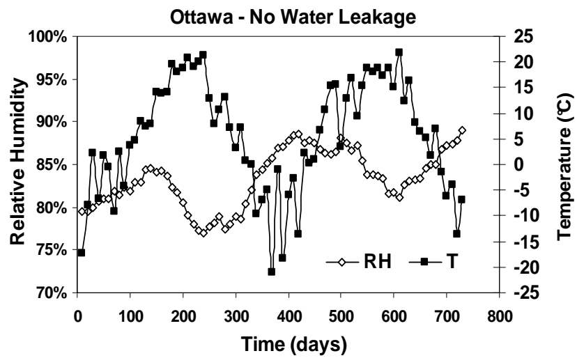
Figure 5 – RH and T variation with time at the region of focus for stucco wall with no water leakage (‘region of focus’ - ‘OSB layer facing stud cavity’)
